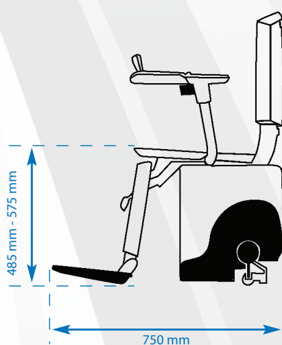
SIDE - Unfolded
