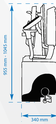
SIDE - Folded
