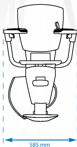
FRONT - Unfolded
